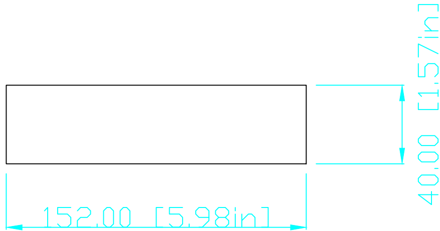
Short side outline: 40mm X 152mm
